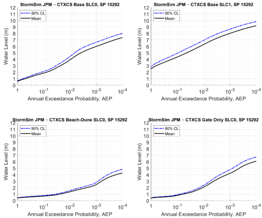
Figure 2-24: Hazard curves for 4 scenarios for SP 15292 (Galveston Mid Bay)
