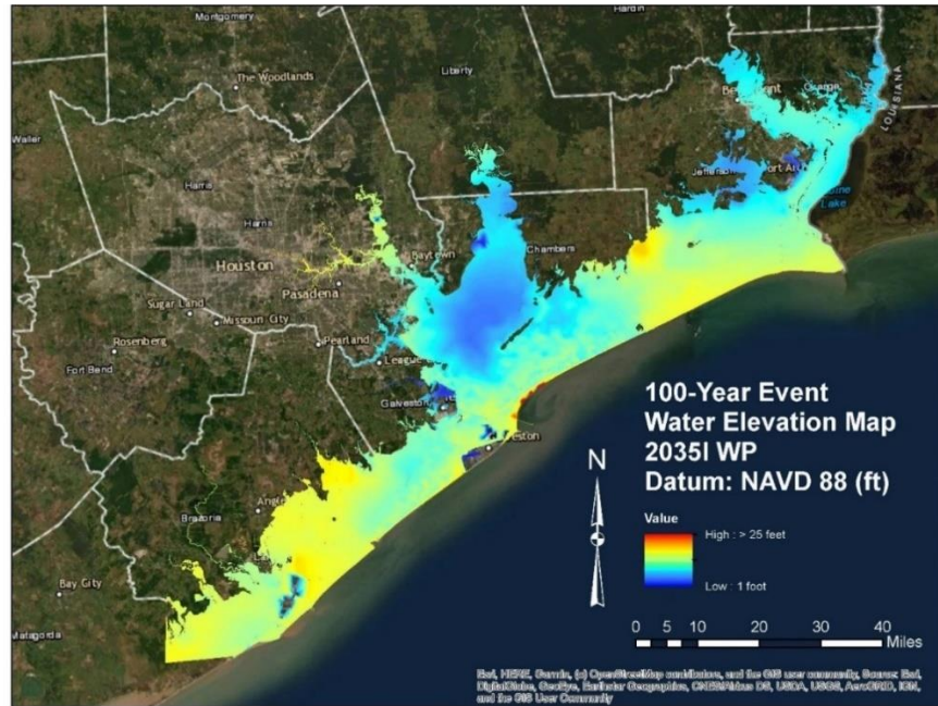
Figure 2-26: 1% AEP SWL (With-Project, Year 2035, Intermediate RSLC)
