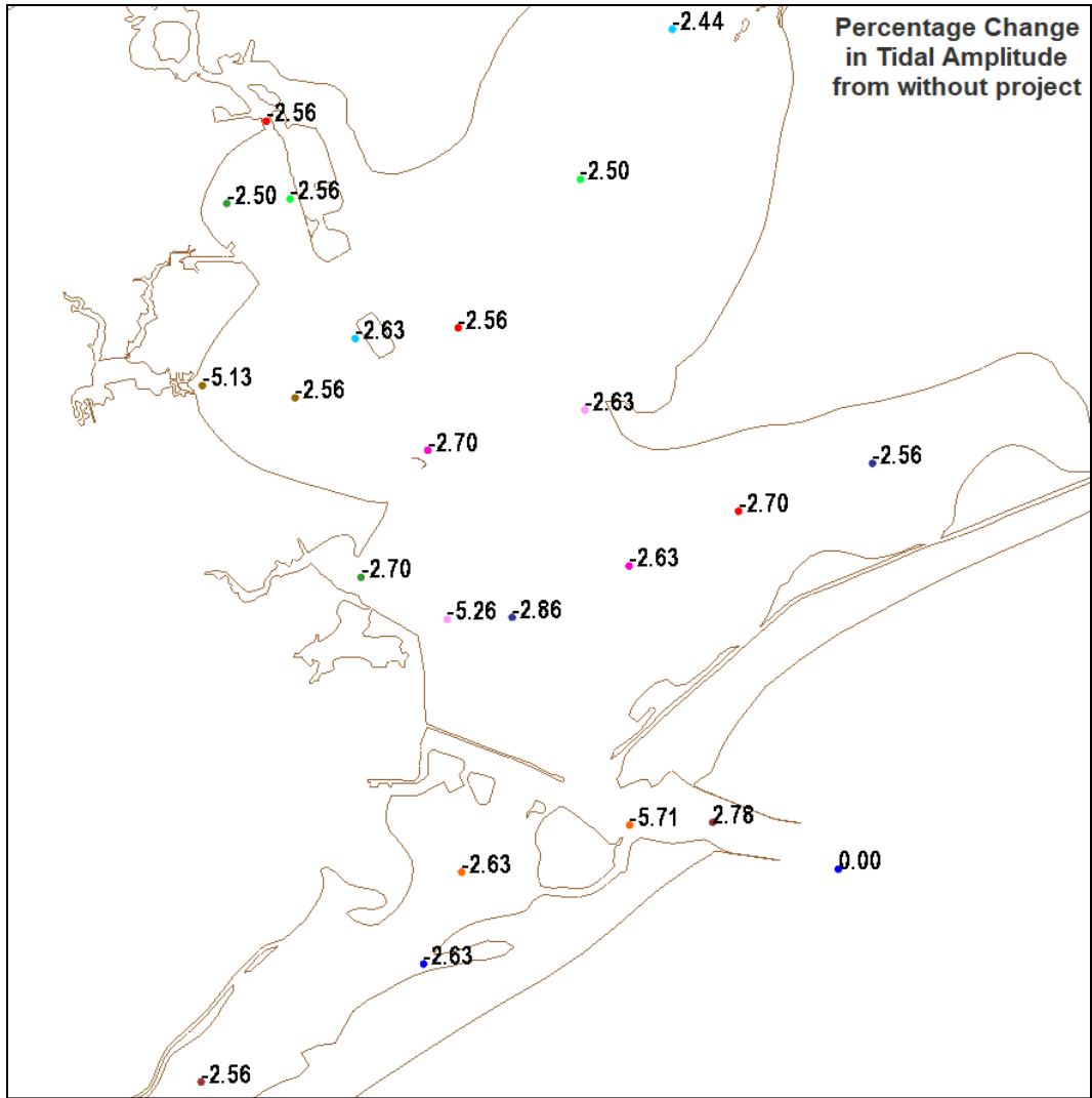
Figure 2-45: Percent Change in Tidal Amplitude for 2019PWP from PWOP
