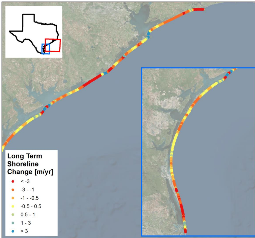
Figure 2-7: Long-term Shoreline Change along the Texas Coast (Paine et al., 2014)
