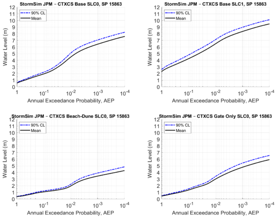
Figure 2-23: Hazard curves for 4 scenarios for SP 15863 (Clear Lake Area)
