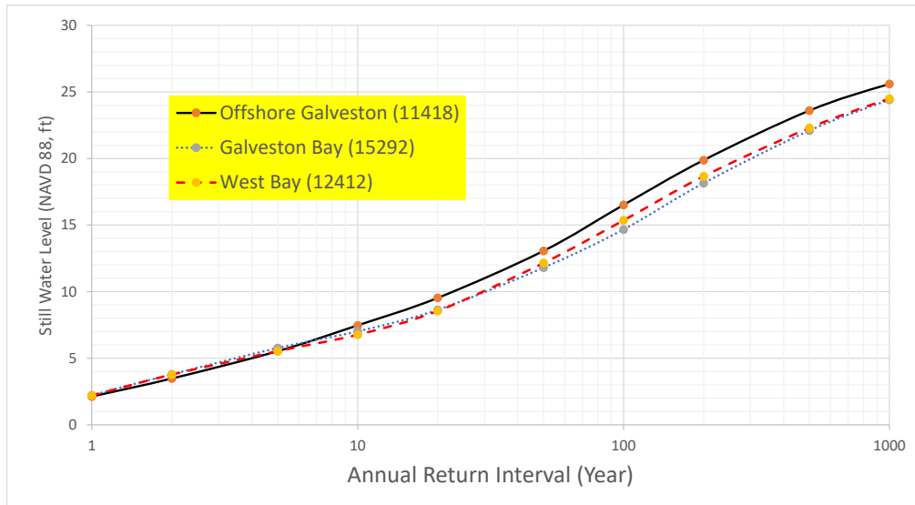
Figure 2-22: Hazard curves at 90% Confidence Interval (CI) at representative stations (Present RSLC scenario- SLC0 condition)
