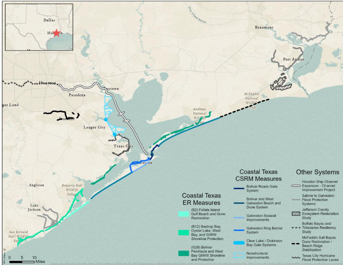
Figure 1-2: General Layout of the Tentatively Selected Plan (Region 1)
