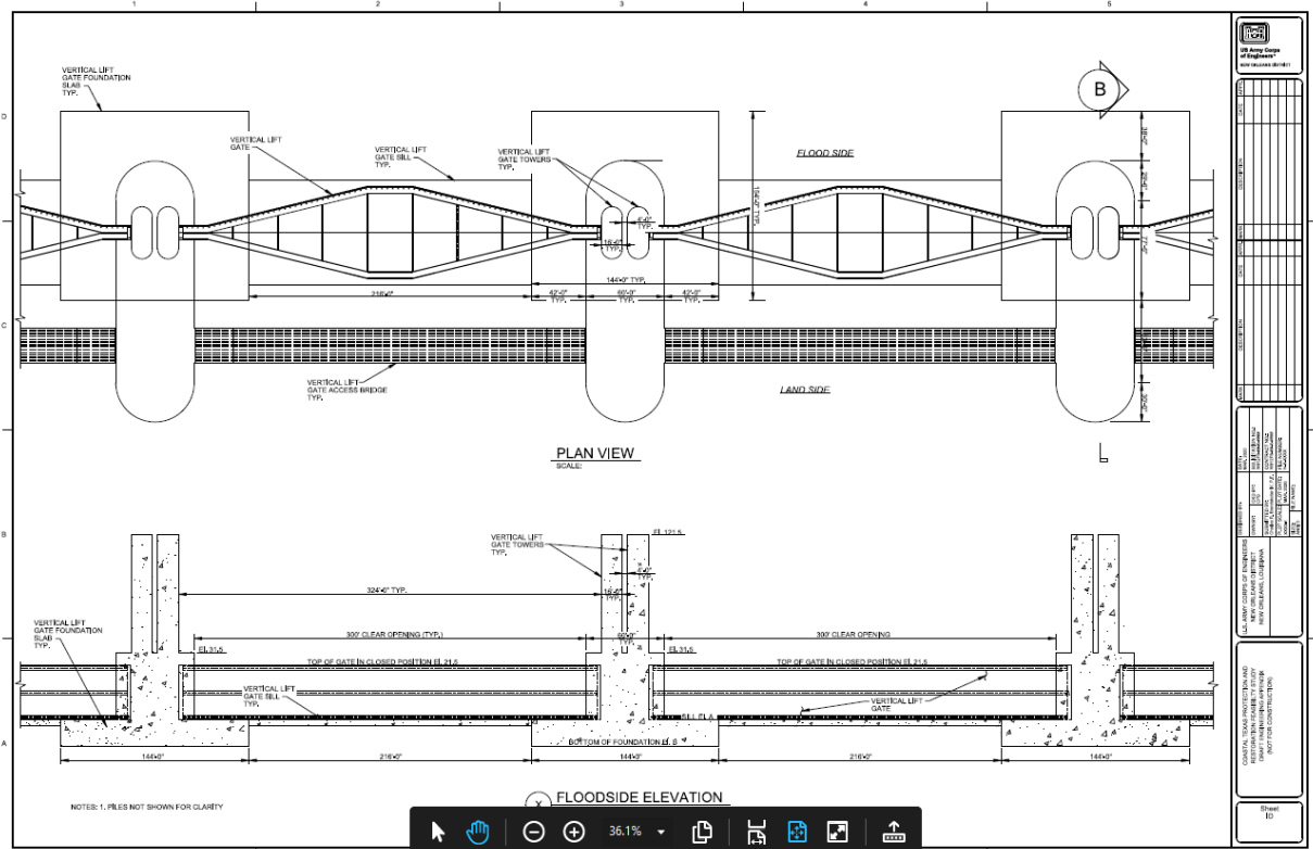
Figure 6-8: Vertical Lift Gates (VLGs) (Technical Drawing)
