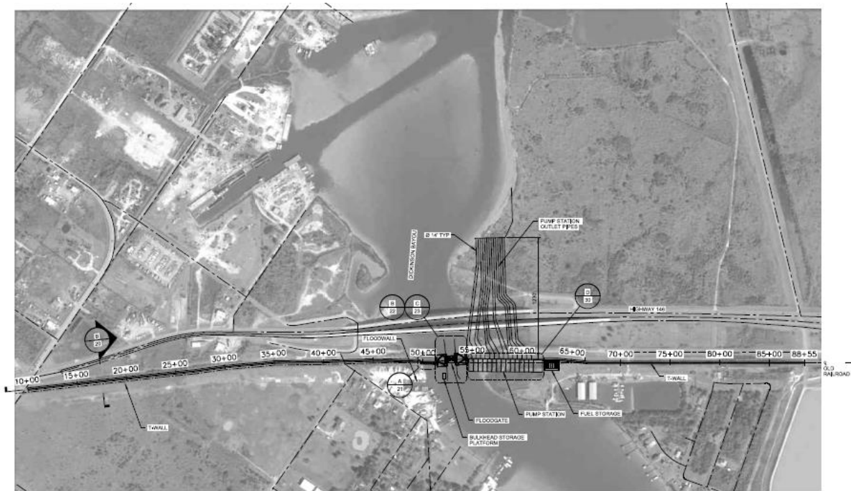
Figure 2-40: Dickinson Bay Gate Closure System with Pump Station Footprint (Annex 2, Annex 5)
