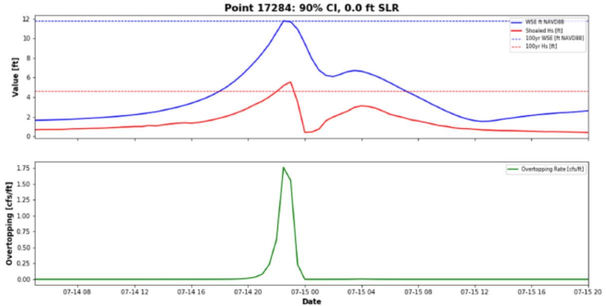
Figure 2-31: Timeseries of water surface elevation and wave heights (top), overtopping rates (bottom)
