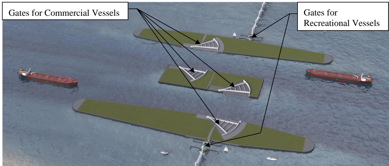
Figure 6-11: Houston Ship Channel Gate Complex (Conceptual Rendition)
