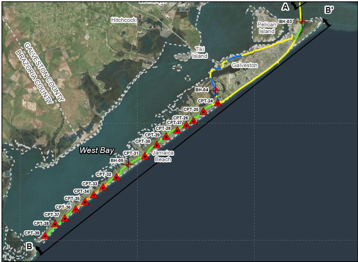
Figure 3-10: Boring Plan on Galveston Island (Sea Wall to San Luis Pass)
