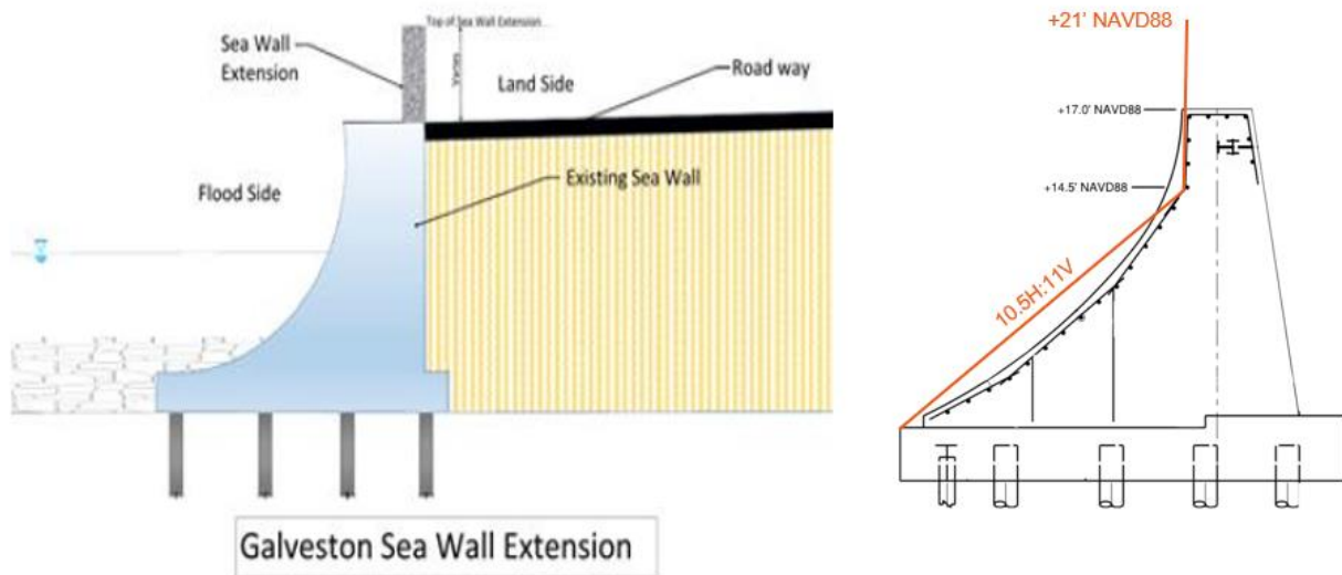
Figure 2-35: Schematics of Seawall Extension
