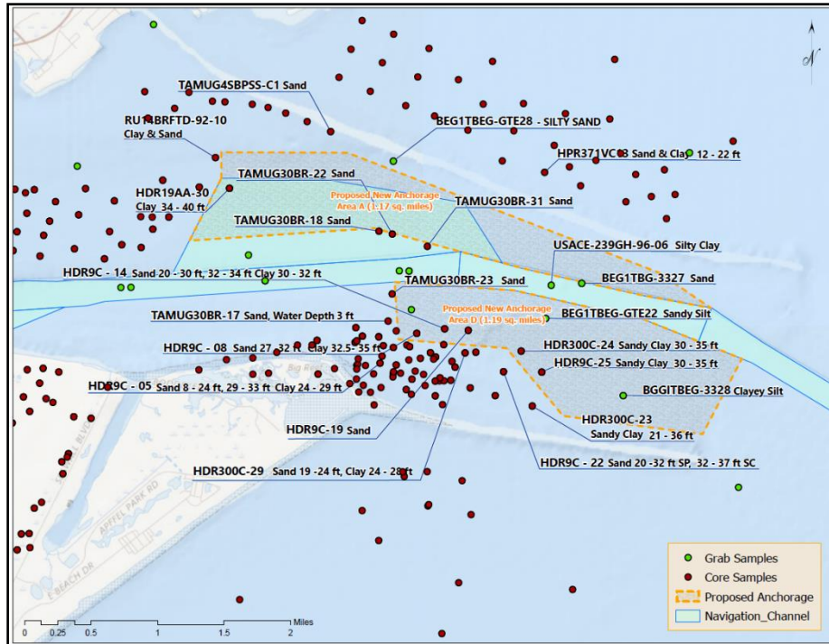
Figure 3-14: Proposed Galveston Harbor Entrance Channel and Anchorage Area Improvements
