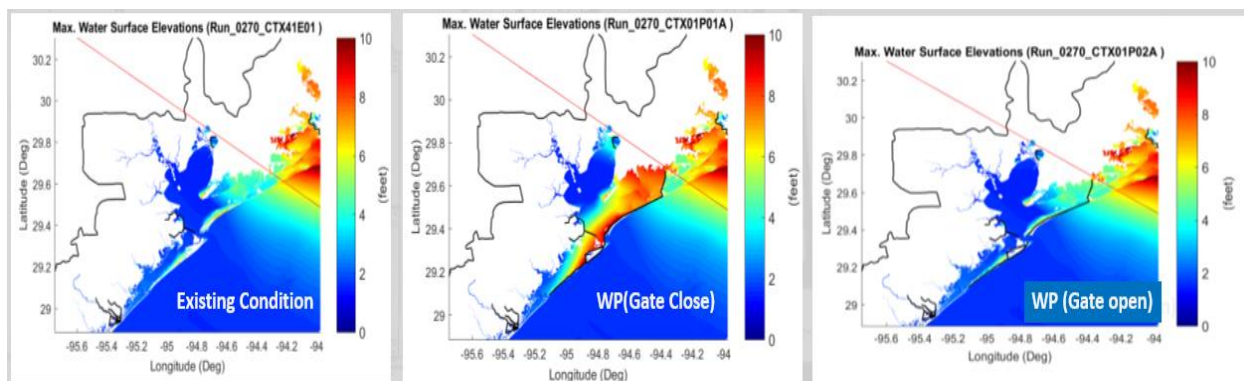
Figure 2-29: Impact of Gate Closure on Storm Track (Storm #270)
