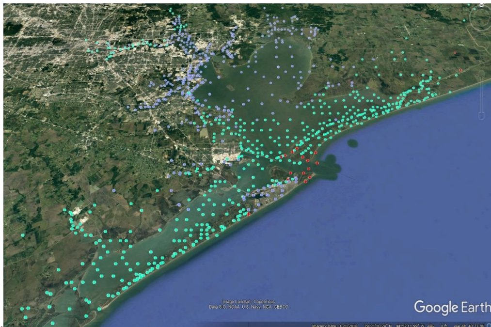
Figure 2-27: WP and WOP SWL Difference Map (1% AEP, Year 2035, Intermediate RSLC)
