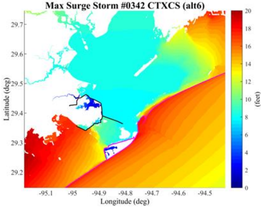
Figure 2-18: Maximum Surge Elevation from Storm Number 342 (With Project)
