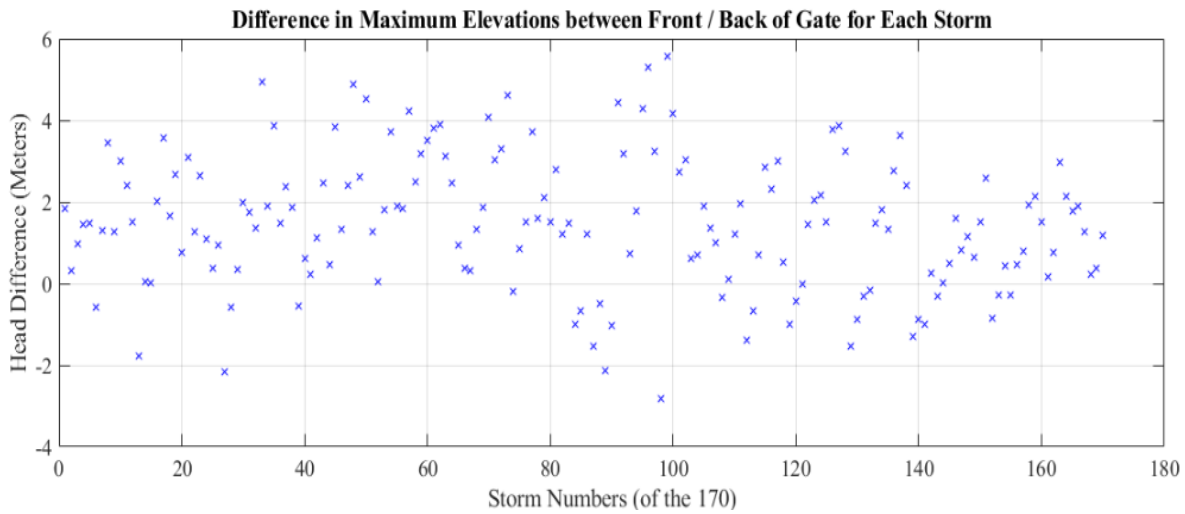
Figure 2-34: Difference in Elevations Between Front and Back Side of Surge Barrier
