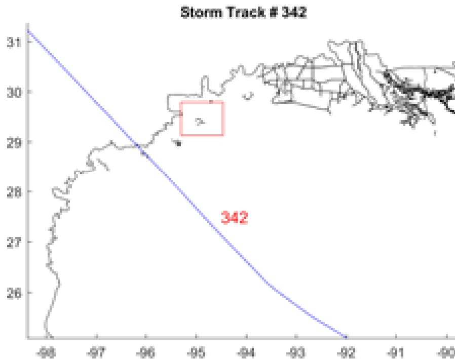
Figure 2-15: Track Time History for Tropical Synthetic Storm Number 342
