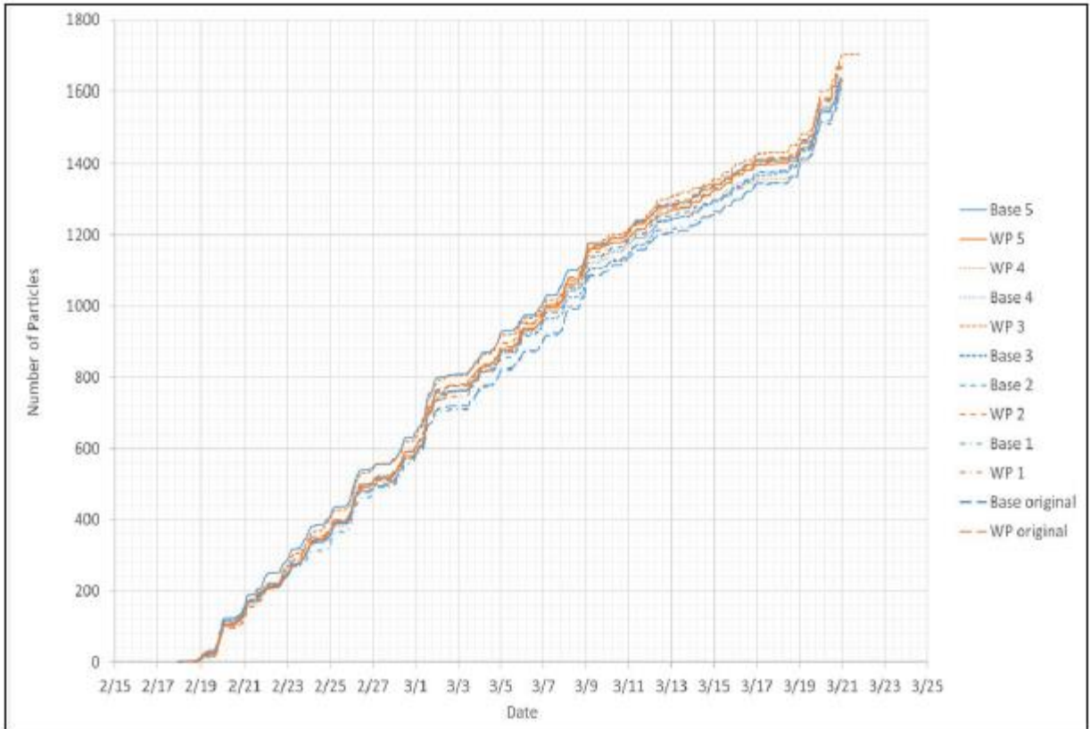
Figure 2-49: Outcome of PTM sensitivity simulations for without-project or base conditions (blue) and with-project conditions (WP) (orange).
