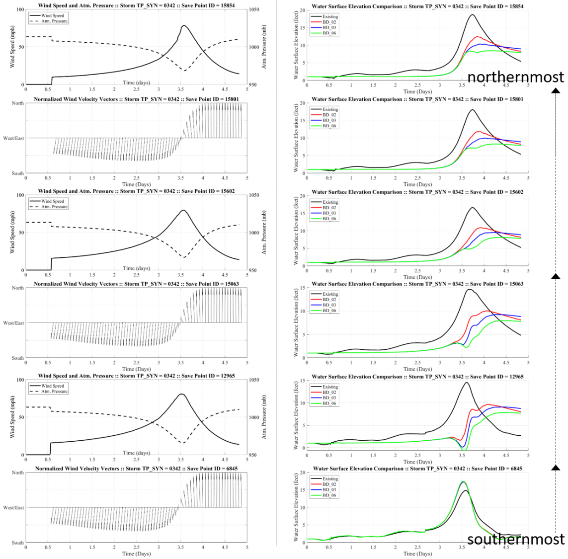
Figure 2-20: Comparison of water surface elevation for storm 342 (right hand side) at six (6) save point locations for four (4) different configurations. The left hand side shows the corresponding wind direction (as normalized vectors), wind speed and atmospheric pressure
