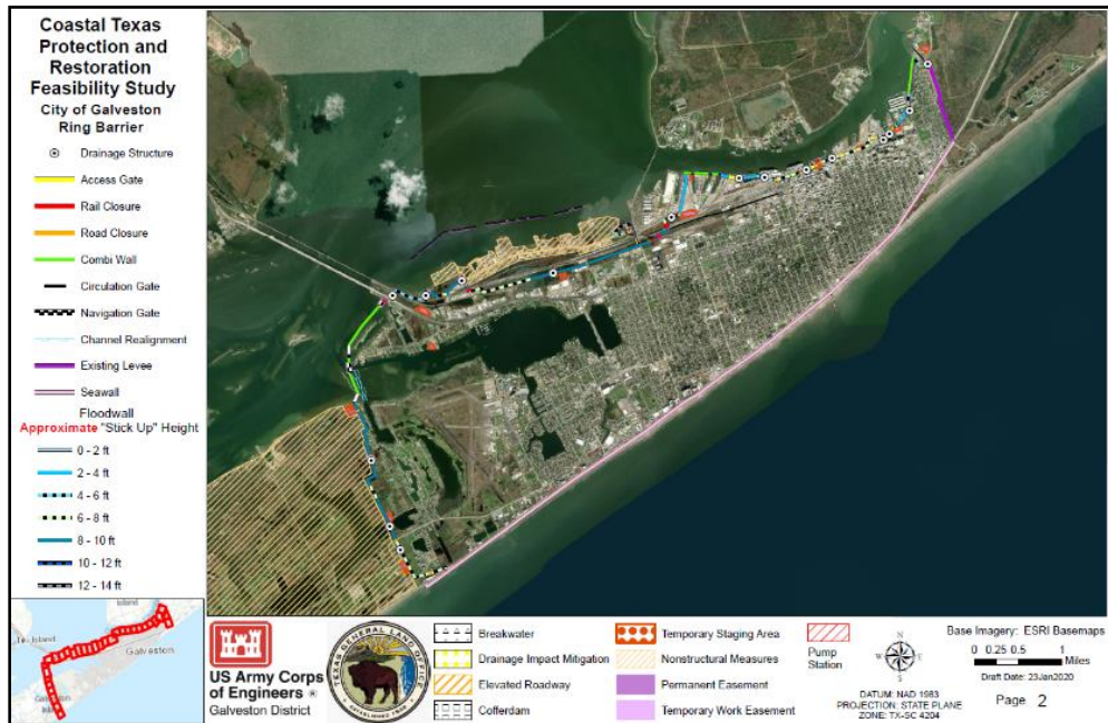
Figure 3-6: City of Galveston Ring Barrier (Outside of Seawall Portion)
