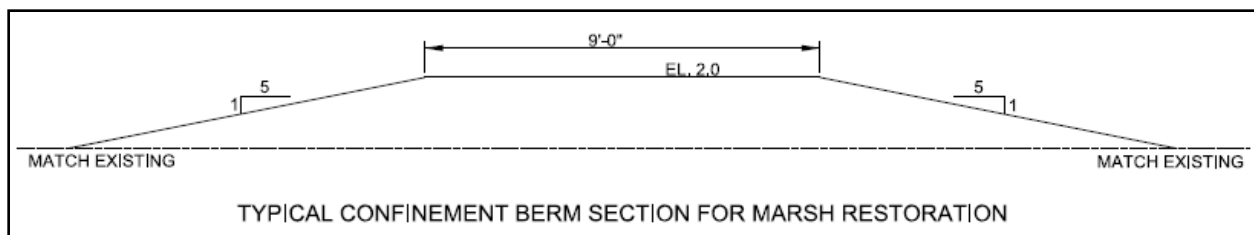
Figure 3-16: Typical Proposed Temporary Confinement Berm Section for Marsh Restoration
