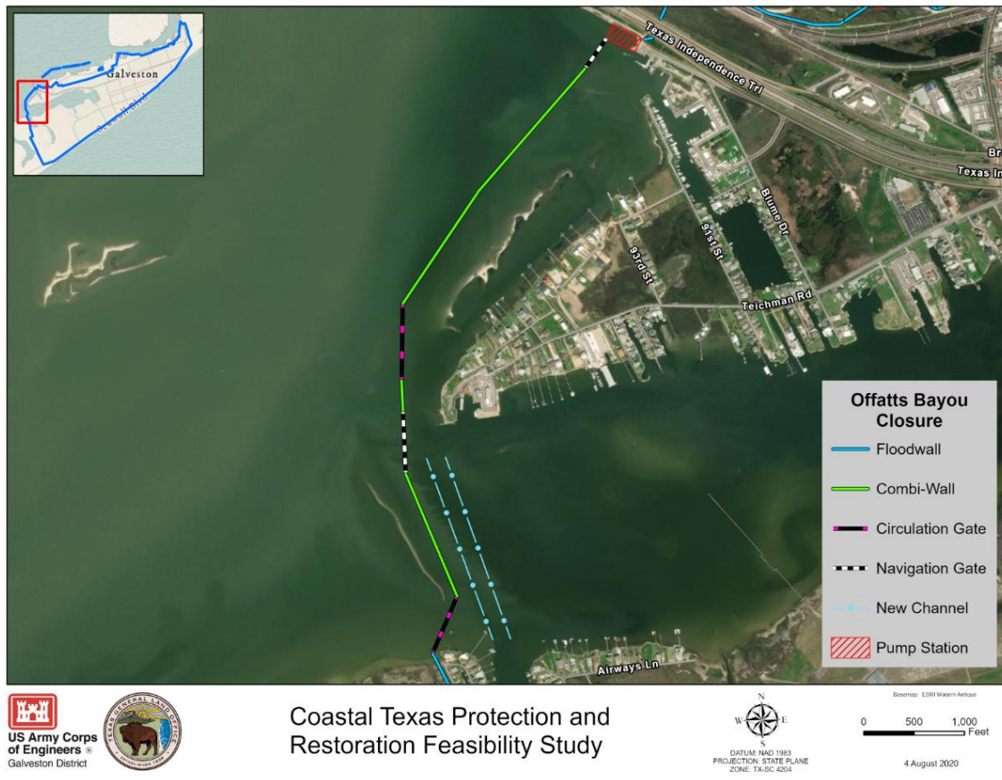
Figure 4-13: Offatts Bayou Crossing
