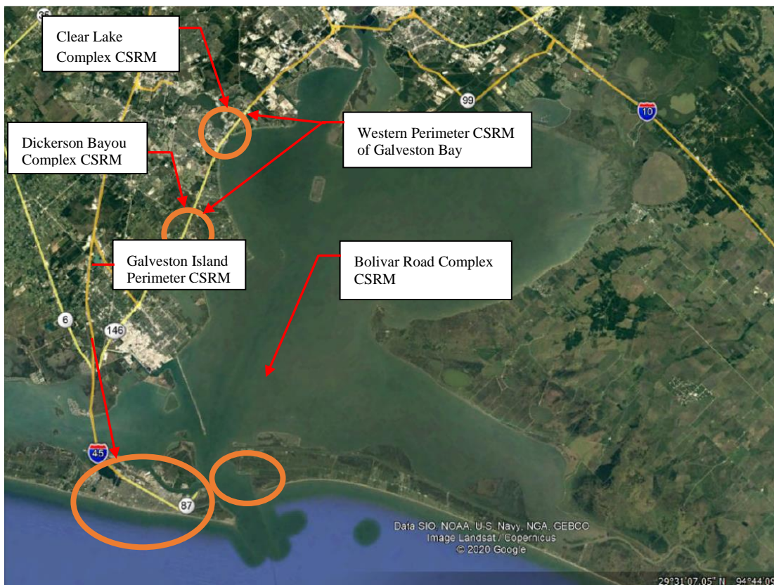
Figure 6-1: Overall Structural Feature Map
