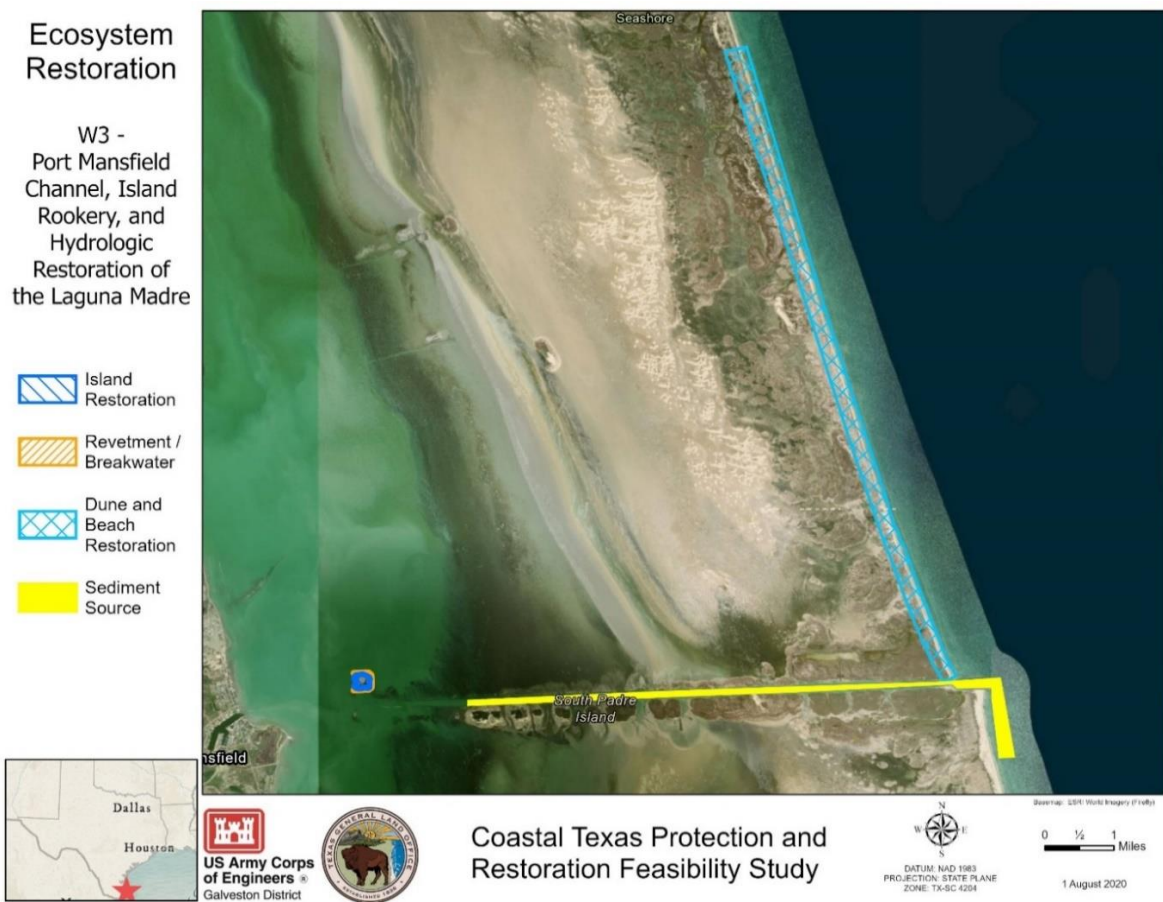
Figure 7-9: W-3 – Port Mansfield Channel, Island Rookery, and Hydrologic Restoration
