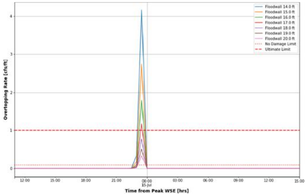
Figure 2-32: GRBS System Height Sensitivity on RSLC Scenario
