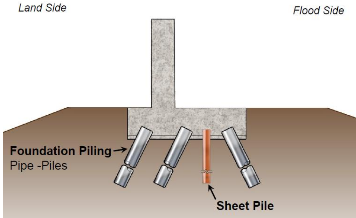
Figure 6-15: Typical Floodwall Section for the GRBS
