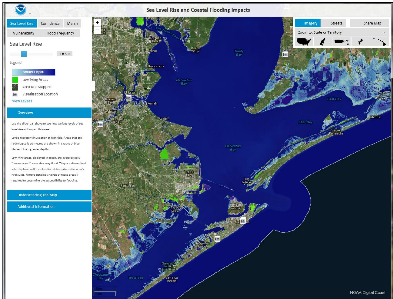
Figure 2-14: Extent of Inundation at Galveston, Texas with 2-foot Sea Level Rise Scenario from Present Condition
