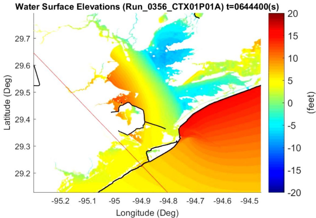
Figure 2-33: Variations in With-Project SWL
