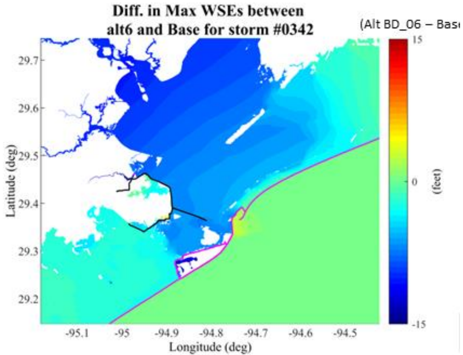
Figure 2-19 : Difference in SWL for Storm 342 Under Without-Project and With-Project Condition.
