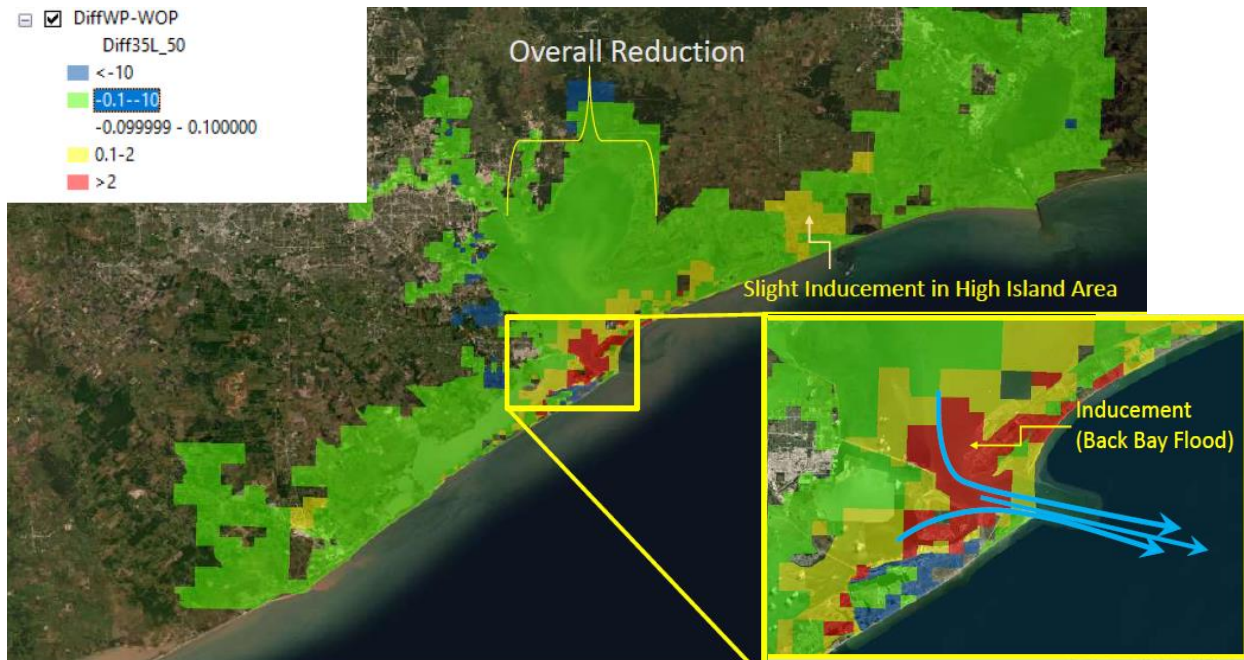
Figure 2-28: WP and WOP SWL Difference Map (0.5% AEP, Year 2035, Intermediate RSLC)
