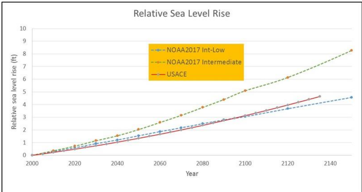
Figure 2-11: Relative Sea Level Rise at Pier 21 Using USACE and NOAA Rates
