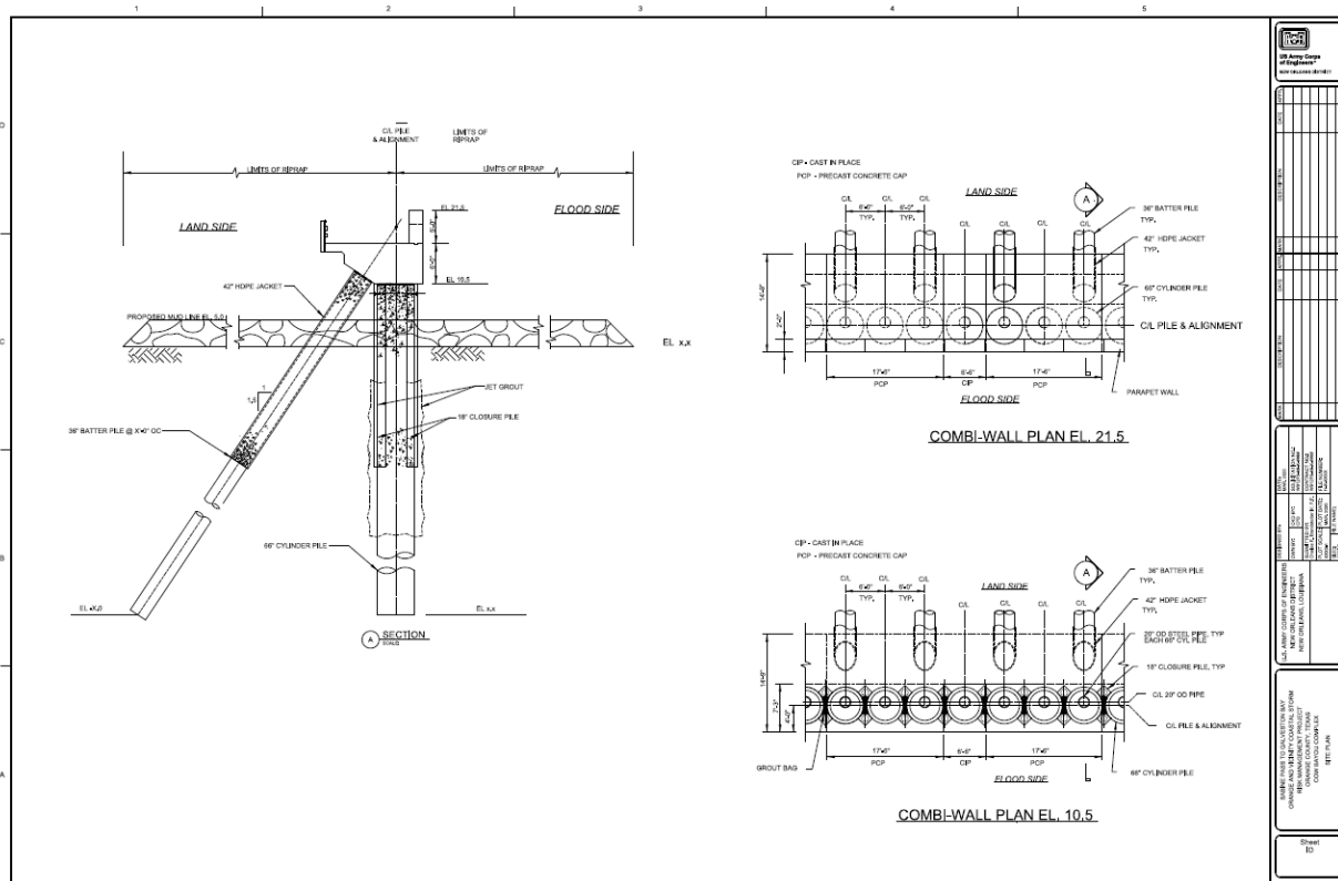
Figure 6-6: Combi-wall (Technical Drawing)
