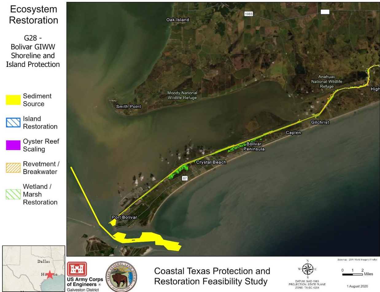
Figure 7-1: G-28 – Bolivar and West Bay GIWW Shoreline and Island Protection East
