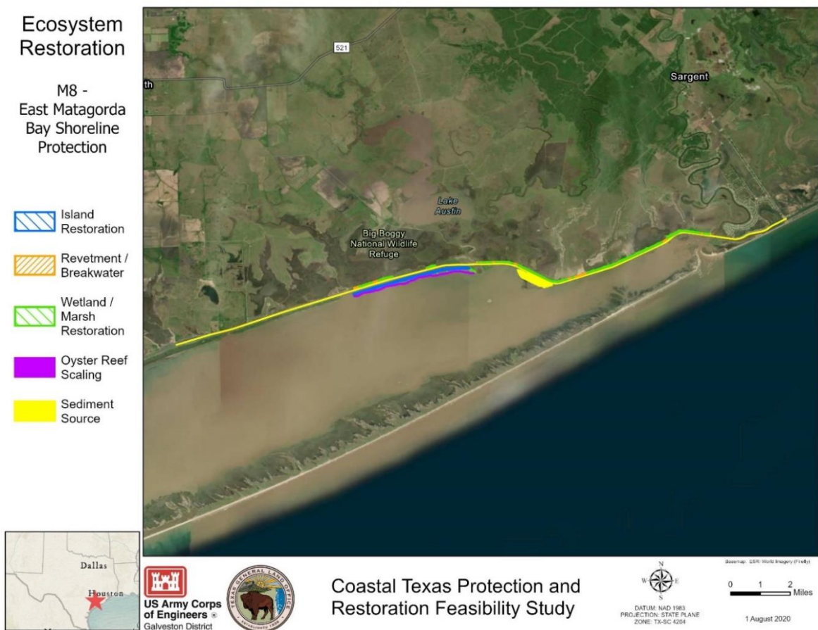
Figure 7-7: M-8 – East Matagorda Bay Shoreline Protection
