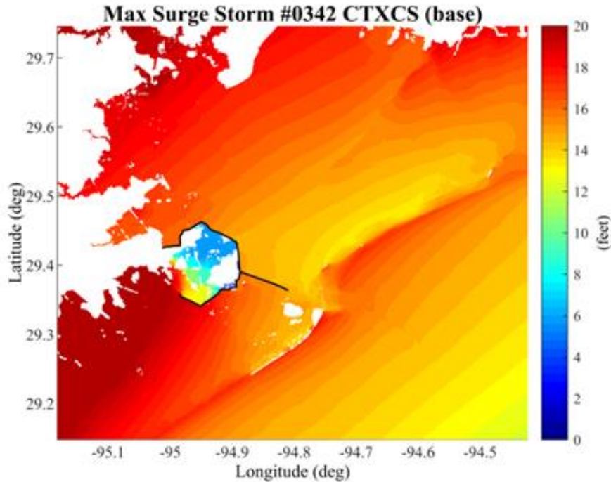
Figure 2-16: Maximum Surge Elevation from Storm #342 (Without Project)
