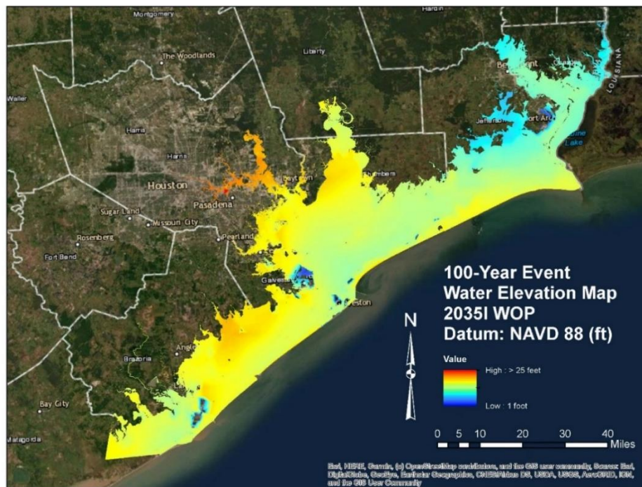
Figure 2-25: 1% AEP SWL (Without Project, Year 2035, Intermediate RSLC)
